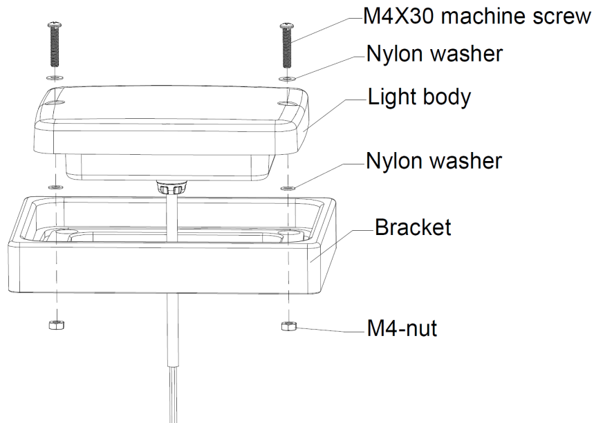
(Installation diagram)
