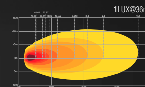
FLOOD BEAM
