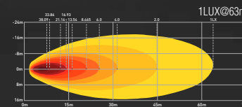
DRIVING BEAM
