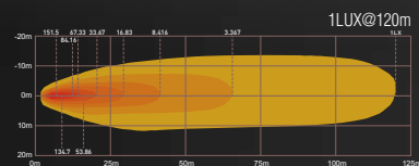
SPOT BEAM
